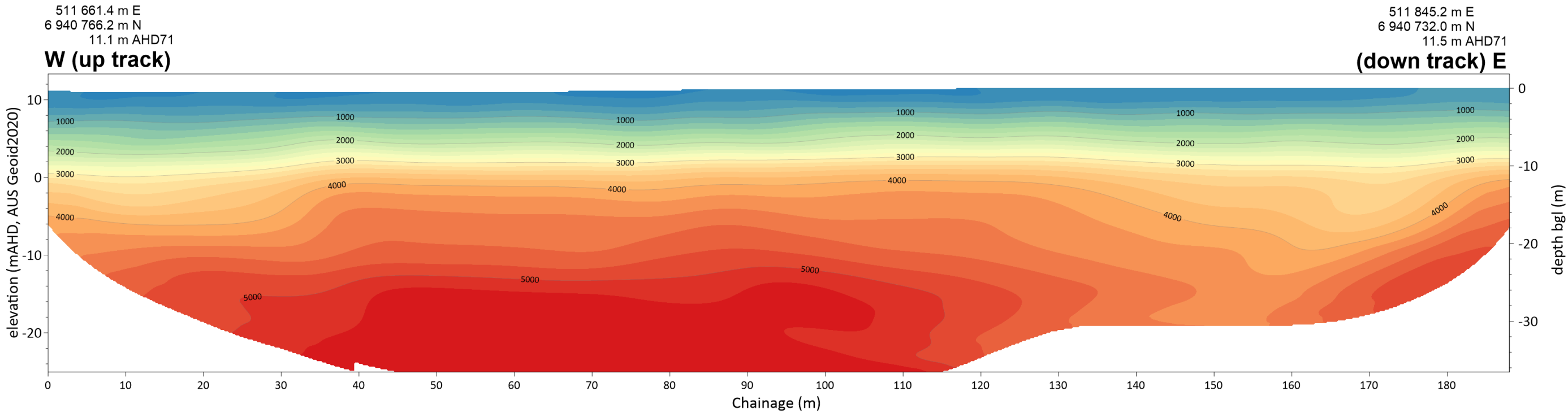
Seismic Line MASW AU-GP 140
